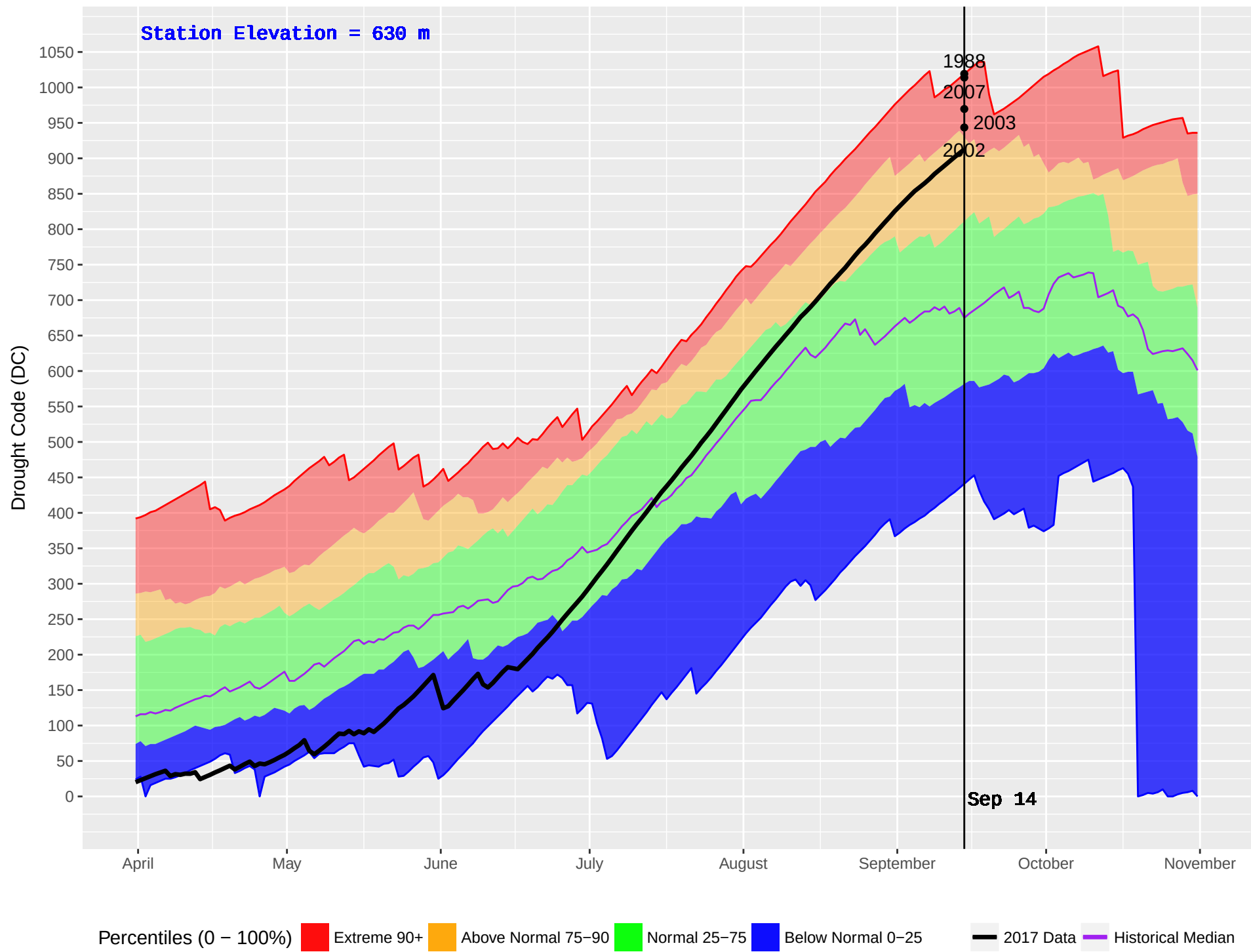
GRAND FORKS (392) : Historical (1981–2016) and Current (2017) Noon Drought Code (DC)
